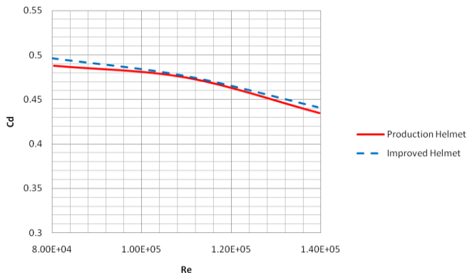
(FIGURE 24) COEFFICIENT OF DRAG VS REYNOLDS NUMBER PITCH ANGLE = -45 DEGREES
