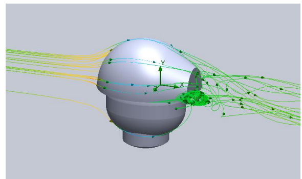
(FIGURE 15) TRUNCATED HELMET FLOW VISUALIZATION
