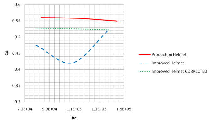
(FIGURE 25) COEFFICIENT OF DRAG VS REYNOLDS NUMBER PITCH ANGLE = -90 DEGREES
