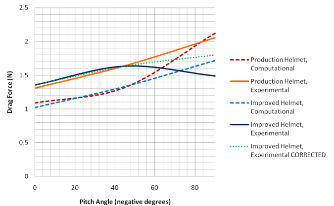
(FIGURE 26) DRAG FORCE VS PITCH ANGLE 11.2 M/S
