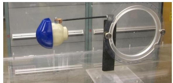
(FIGURE 22) IMPROVED HELMET AT PITCH ANGLE = -90 DEGREES
