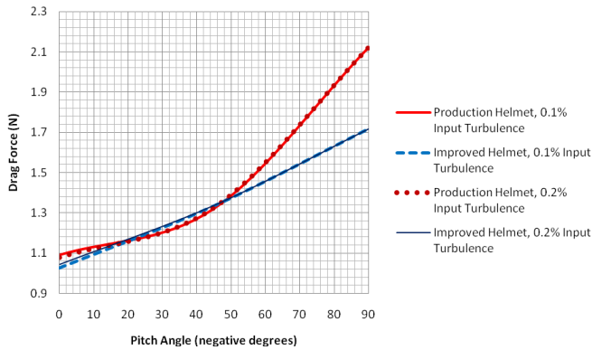
(FIGURE 19) DRAG FORCE VS PITCH ANGLE, INPUT TURBULENCE COMPARISON
