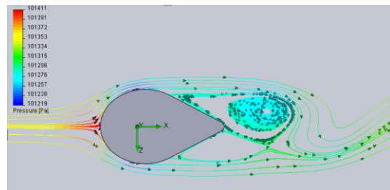
(FIGURE 2) PRODUCTION HELMET FLOW VISUALIZATION
