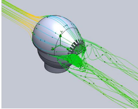
(FIGURE 16) VENTED BASE CAVITY FLOW VISUALIZATION
