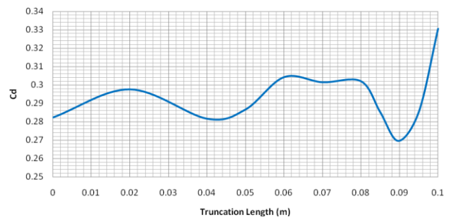
(FIGURE 14) COEFFICIENT OF DRAG VS TRUNCATION LENGTH, 11.2 M/S, 0 DEGREE PITCH ANGLE
