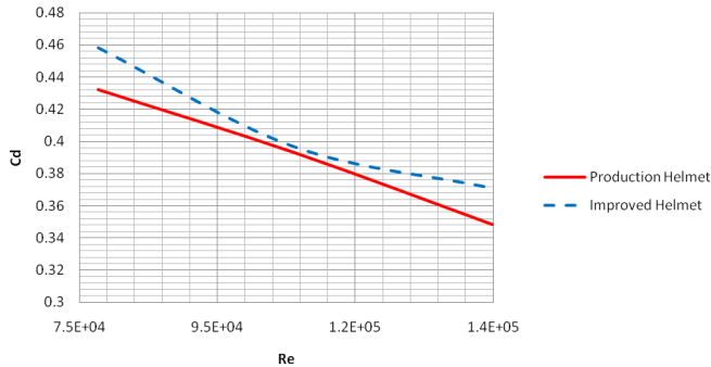
(FIGURE 23) COEFFICIENT OF DRAG VS REYNOLDS NUMBER PITCH ANGLE = 0 DEGREES
